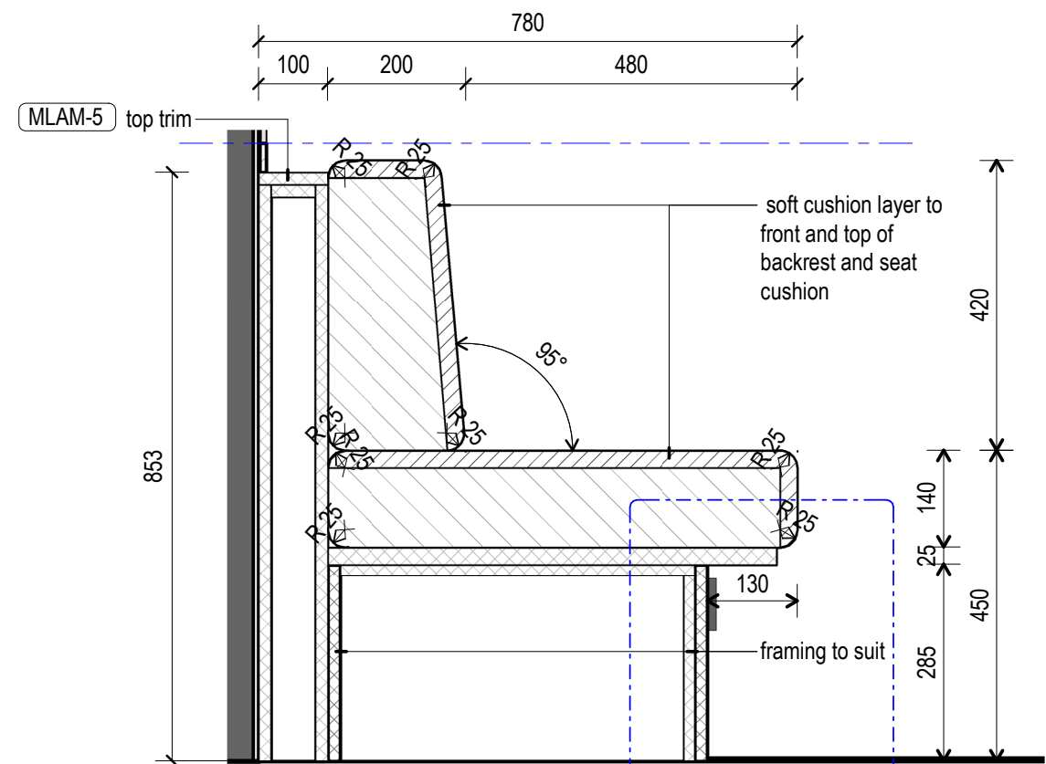
10 JO-SE-2 Detail 1:10
