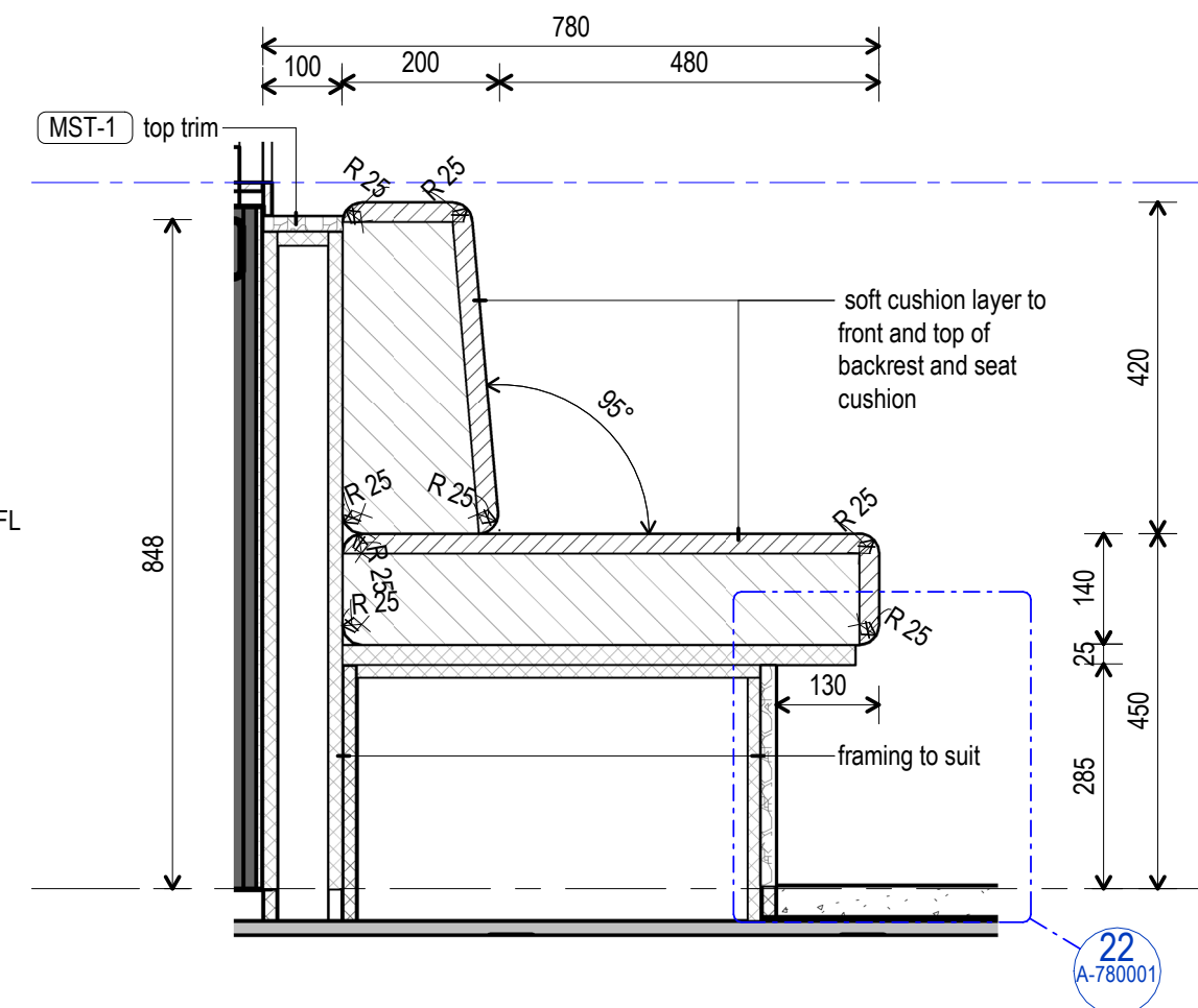
5 JO-SE-1 Detail 1:10
