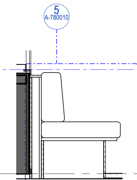
4 JO-SE-1 Section 1:20
