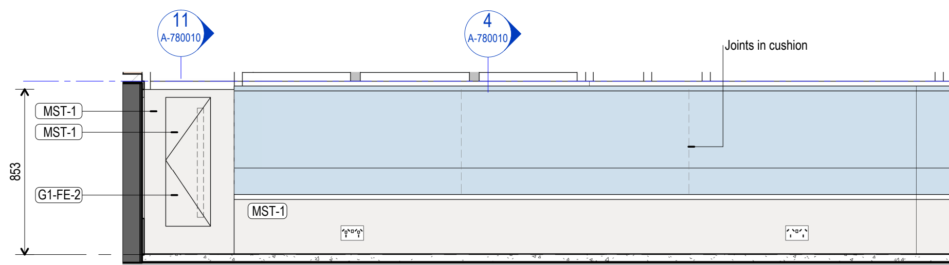
3 JO-SE-1 & JO-ST-3 Elevation 1:20
