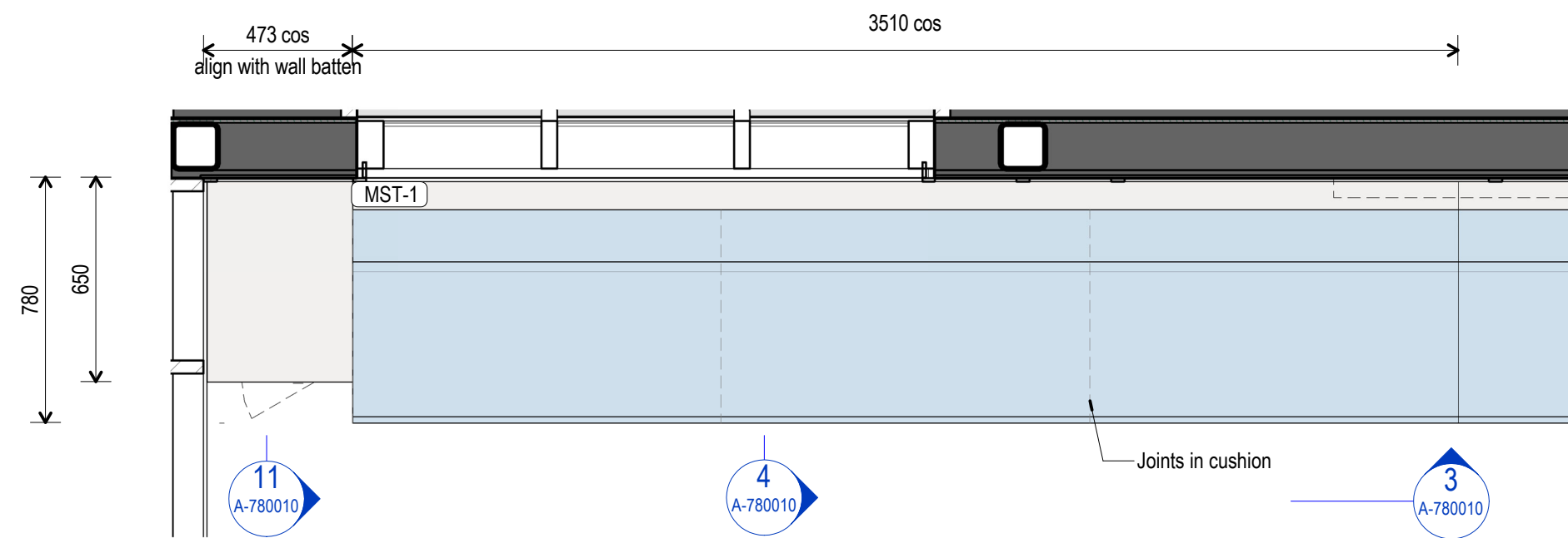
2 JO-SE-1 & JO-ST-3 Plan 1:20
