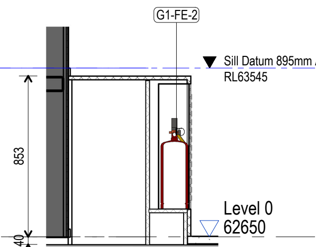
11 JO-ST-3 Section 1:20
