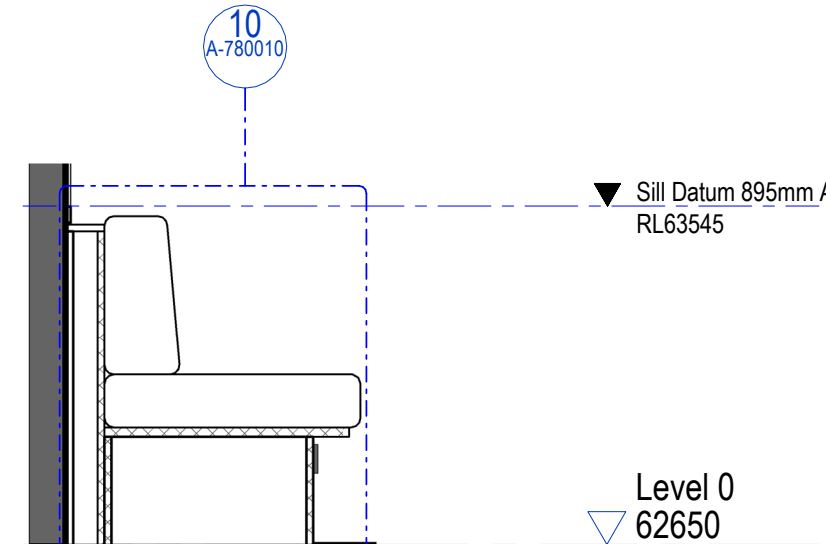
41 JO-SE-2 Section 1:20
